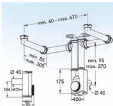
Siphon double Space Saver
